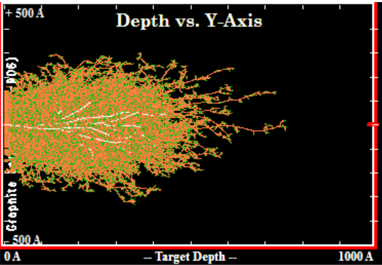
SRIM simulation of 30 keV Ga in graphite
